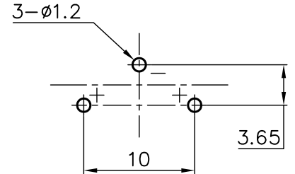
PCB Layout Diagram Top View
